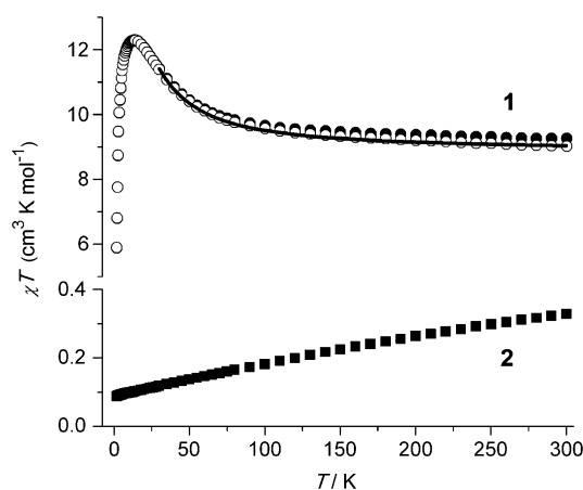
Figure 2. Plots of \chi T values versus temperature ( T ) for polycrystalline samples of 1 (●) and 2 (■), measured in a 0.5 T dc field. Open circles (○) correspond to the \chi T values after subtraction of the \{\text{UO}_2\text{Cd}_2\} data from the \{\text{UO}_2\text{Mn}_2\} data, to which a value of 0.094 \text{ cm}^3 \text{ K mol}^{-1} has been added as the spin-only contribution of the \text{U}^{\text{V}} center. Solid line: the best fit of the data to Equation (1) with J = +7.5 \text{ cm}^{-1} .
