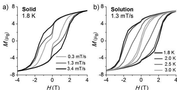
Figure 4. Hysteresis loops for a) the polycrystalline sample of 1 and b) the pyridine solution of 1 , at the indicated temperatures and field sweep rates.
